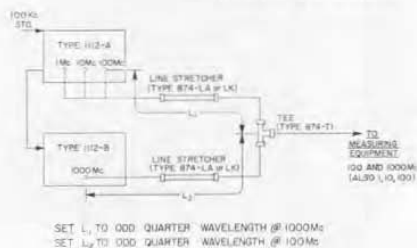
Figure 10. Arrangement for paralleling output signals of Type 1112-A and Type 1112-B Standard Frequency Multipliers using coaxial-line adding network.
