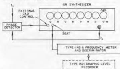
Figure 11. Method of tracking and recording the drift of an unknown frequency, f_x .
