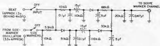
Figure 12. Suggested circuit for generating center-frequency marker and side markers, for use with slow sweeps.
