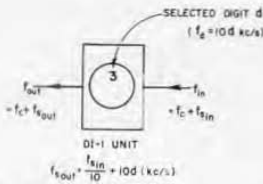
Figure 6. Signal traversing a typical Digit-Insertion Unit.
