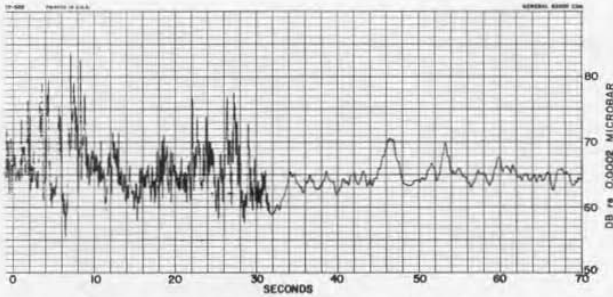
Figure 11. Recording of noise level in a cafeteria with both fast and slow writing speeds and 40-dB potentiometer.
