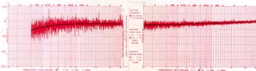
Figure 3. Low-frequency response of the Graphic Level Recorder to \frac{1}{3} -octave band of pink noise, with a writing speed of 1 in/sec.
