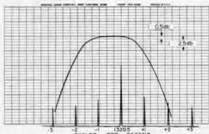
Figure 13. 3-cycle pass band of the Type 1900-A Wave Analyzer recorded by the Type 1521-B Graphic Level Recorder, equipped with an experimental plug-in for generating a sweeping voltage. Frequency markers were generated automatically by use of the circuit shown in Figure 12.
