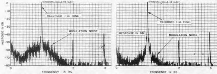
Figure 9. Charts of modulation noise on a 1-kc tone for two different types of magnetic tape. Note that one is about 10 dB better than the other. Such measurement can be made easily with the recording analyzer, owing to the 80-dB dynamic range. For these records, chart speed was 2.5 inches per minute; writing speed, 10 inches per second; bandwidth, 10 c/s.
