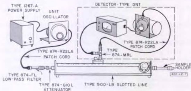
Figure 2. Setup for dielectric measurements.
