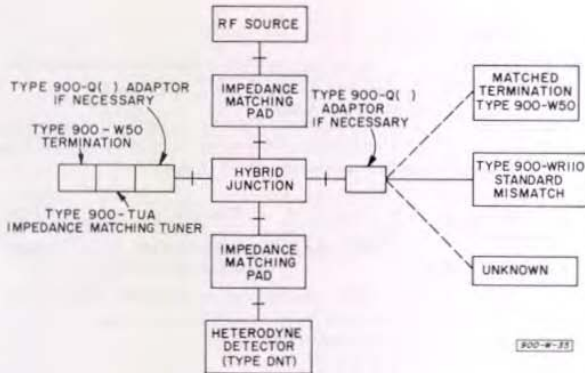
Figure 4. Fixed-frequency reflectometer for measuring VSWR's below 1.1.
