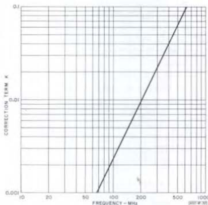
Figure 11. Correction term, K, for Type 900-WO4 Open-Circuit Termination.
