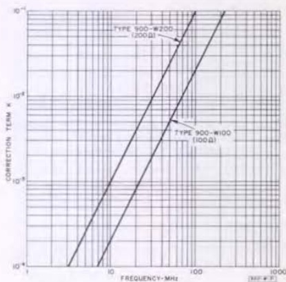
Figure 7. Correction term, K, for the 4-cm difference between the GR900 Connector reference plane and the effective position of the resistance.
